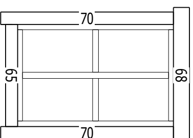
WINDOW 700X1050
